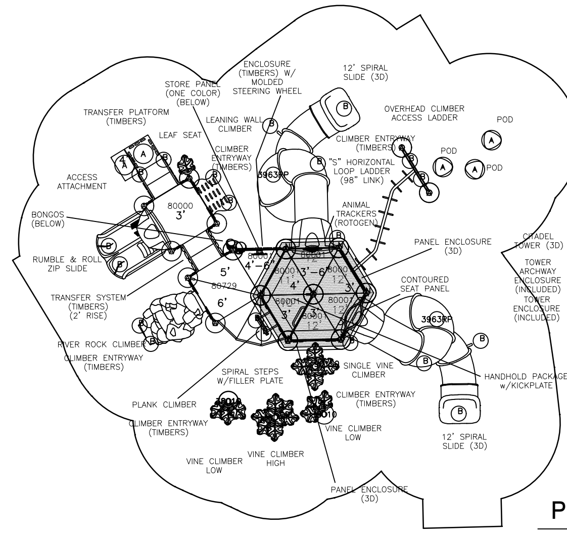
PLAYGROUND FOR CHILDREN 5-12 YEAR OLDS ENLARGED PLAN No Scale
