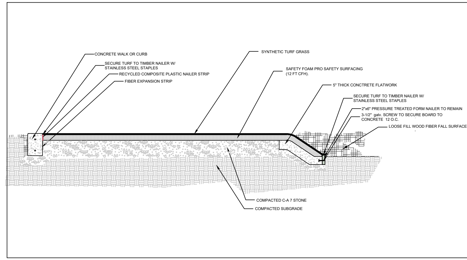
2 1 SYNTHETIC TURF / LOOSE FILL FIBER FALL SURFACE DETAIL No Scale
