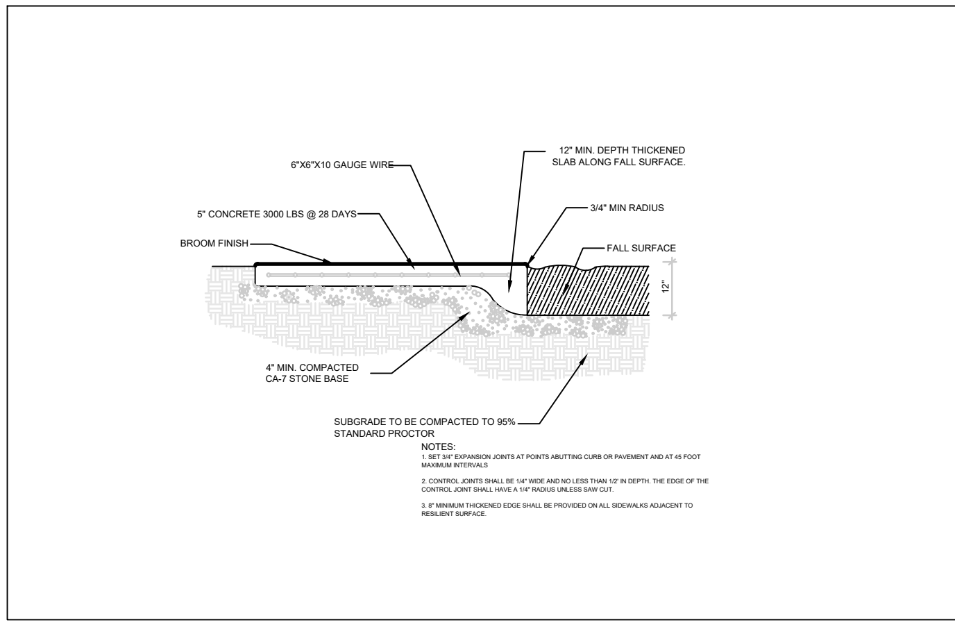
1 1 SIDEWALK DETAIL AT PLAYGROUND No Scale
