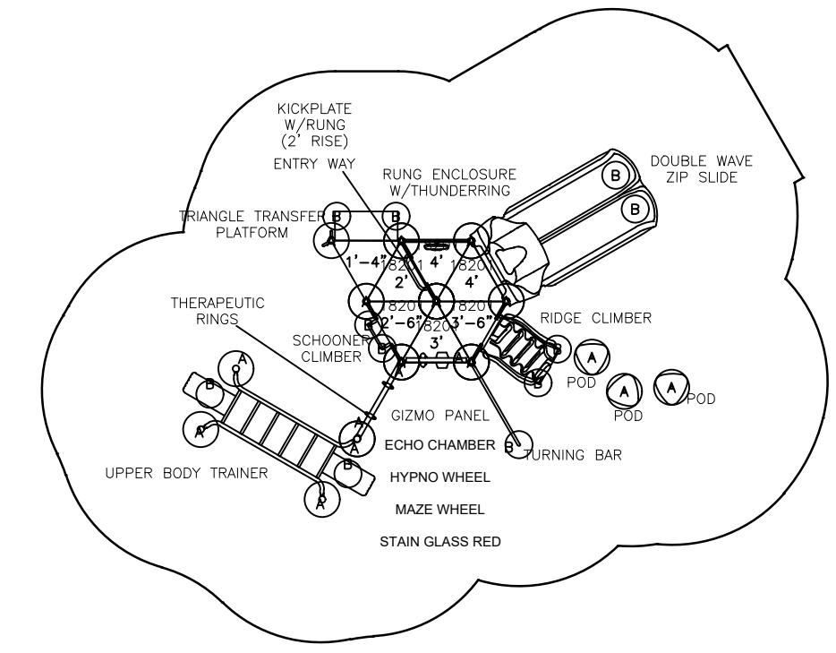
PLAYGROUND FOR CHILDREN 2-5 YEAR OLDS ENLARGED PLAN No Scale
