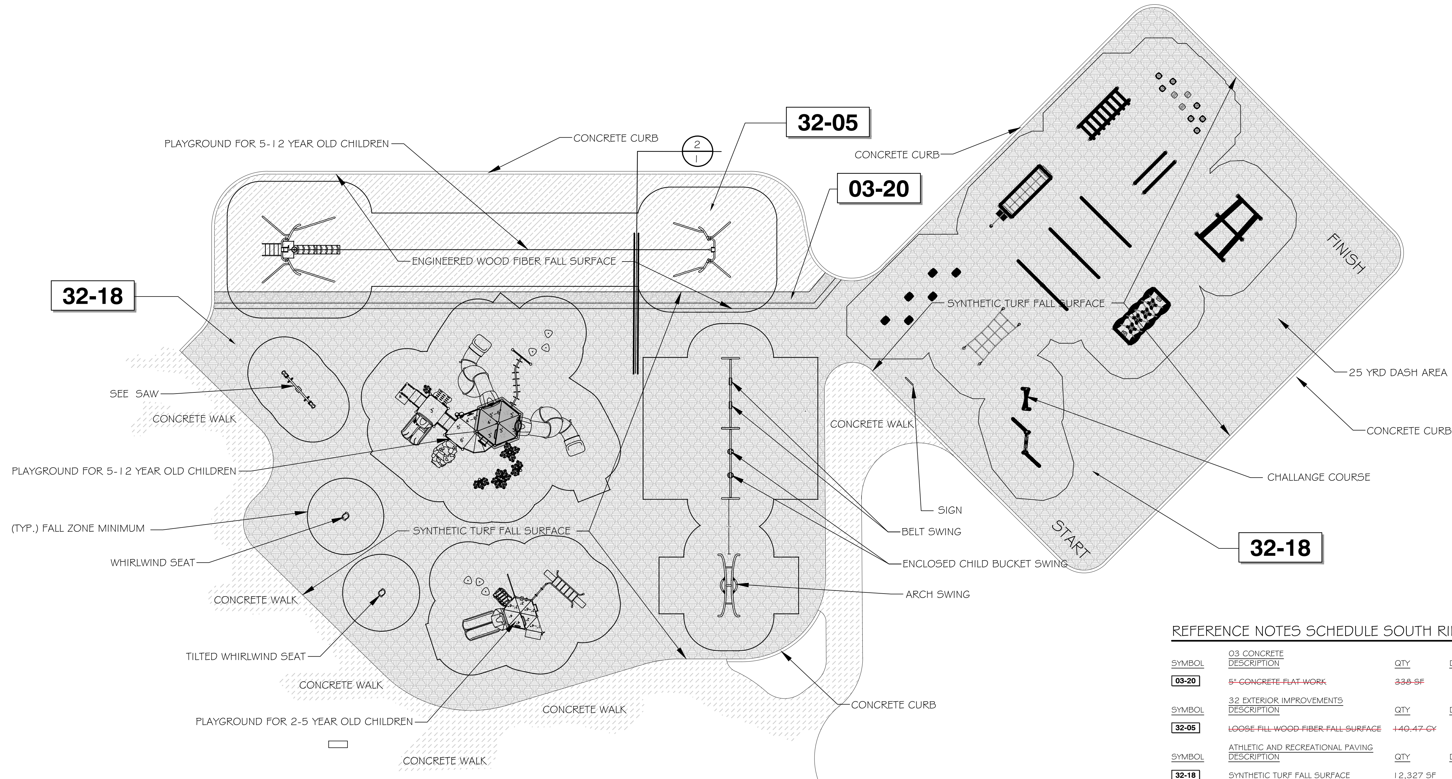
PLAYGROUND FOR CHILDREN 5-12 YEAR OLDS ENLARGED PLAN No Scale
