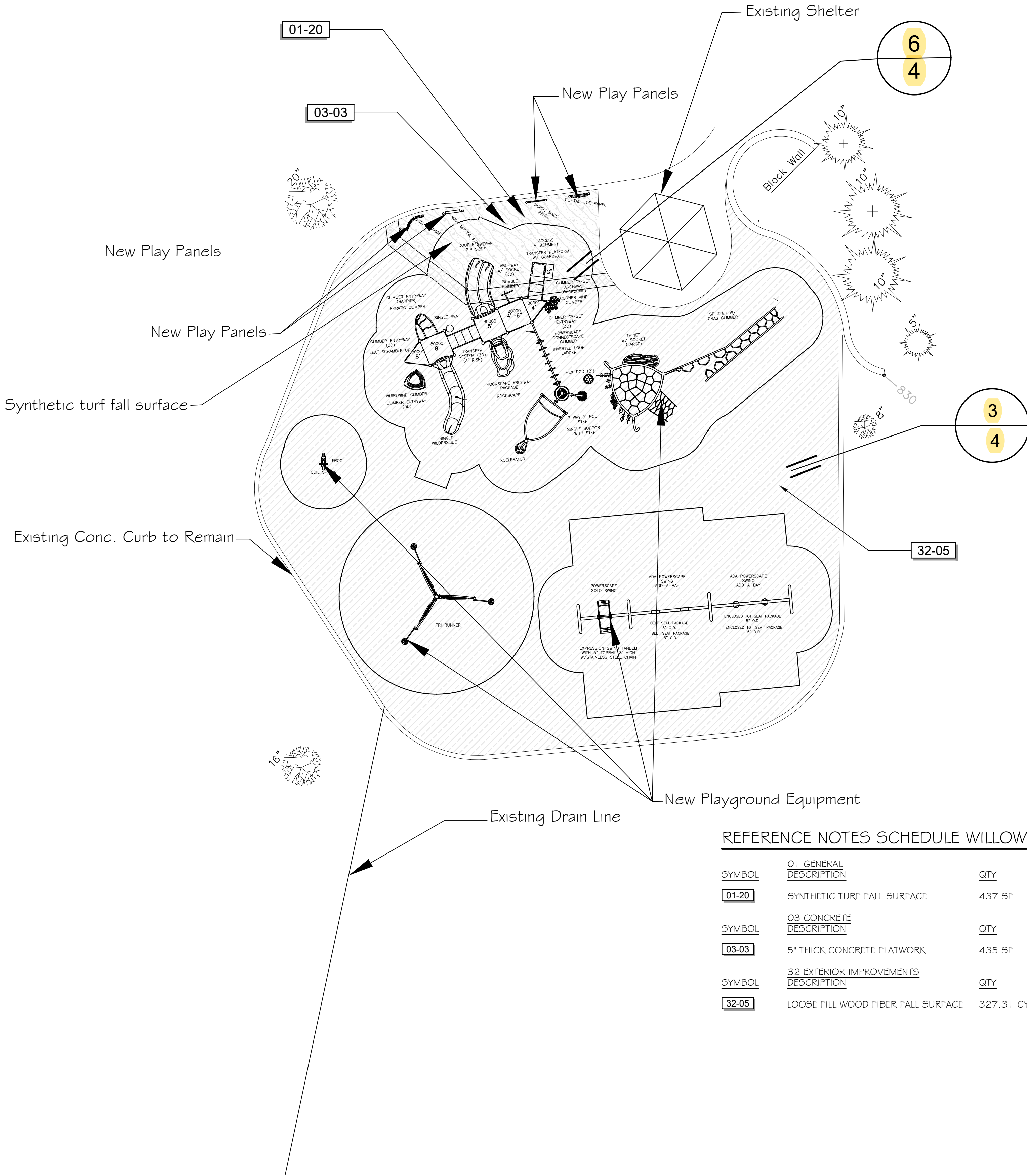
WILLOW PARK NEW PLAYGROUND OVERALL PLAN SCALE 1" = 10 FT
