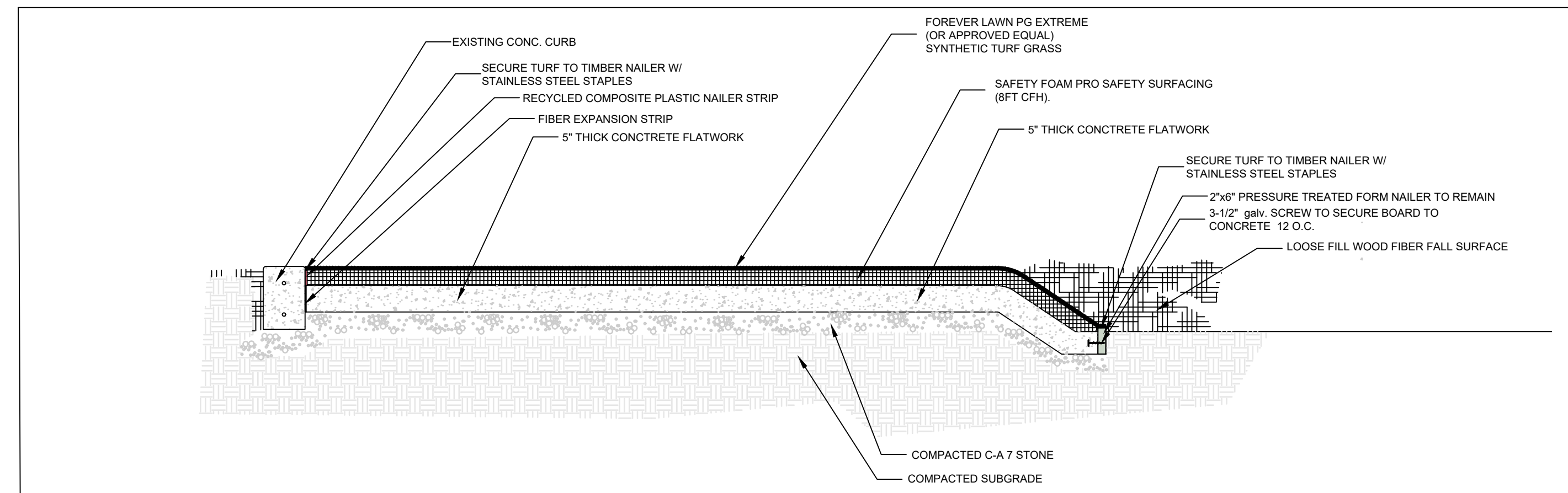
6 SYNTHETIC TURF FALL SURFACE DETAIL
