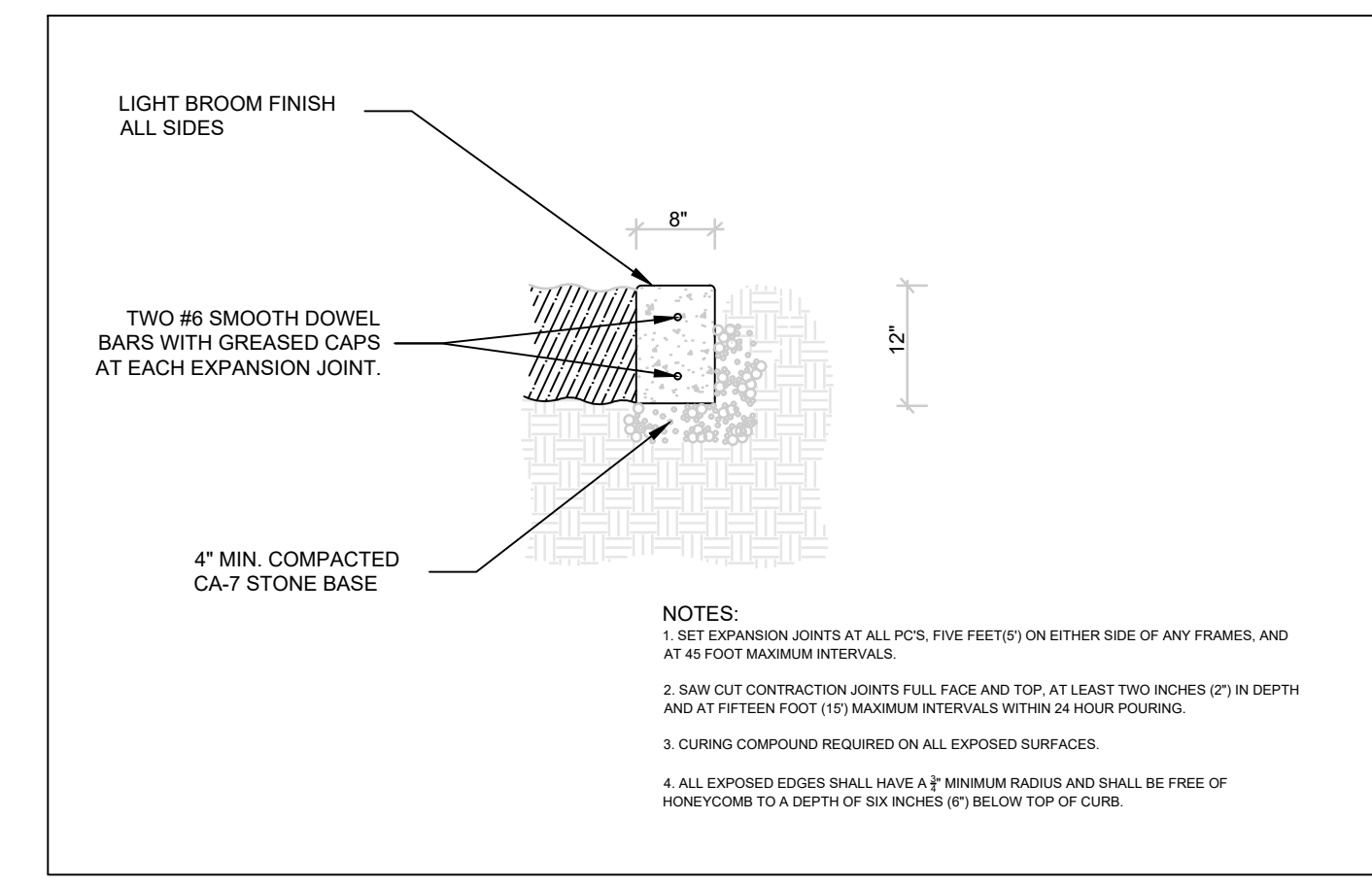
7 4 CURB DETAIL No Scale
