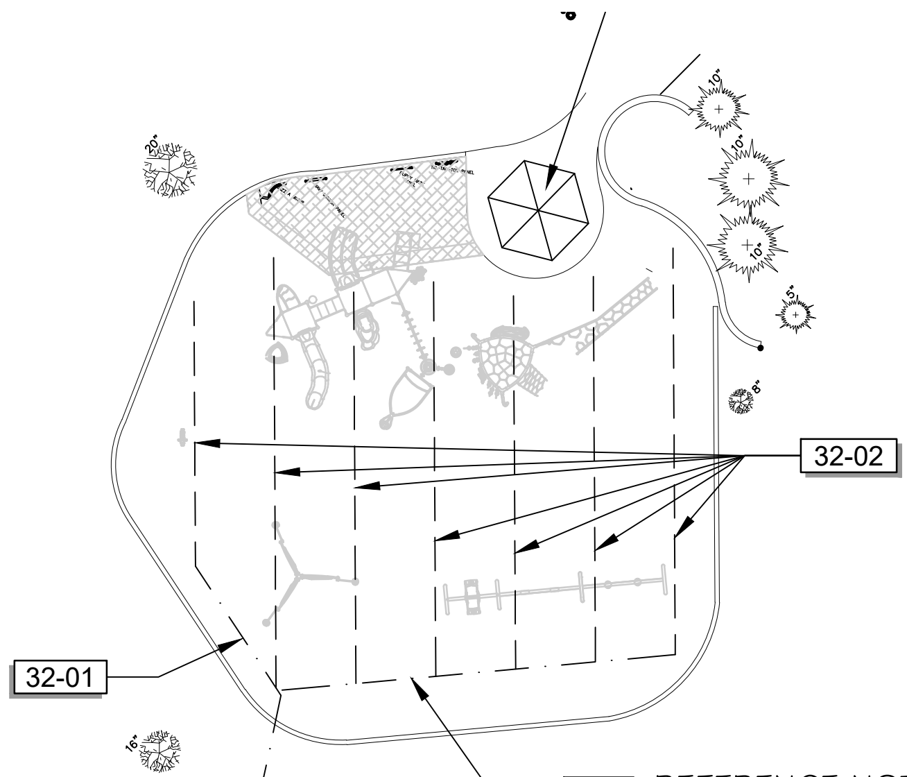
WILLOW PARK PLAYGROUND DEMO PLAN SCALE 1" = 20 FT
