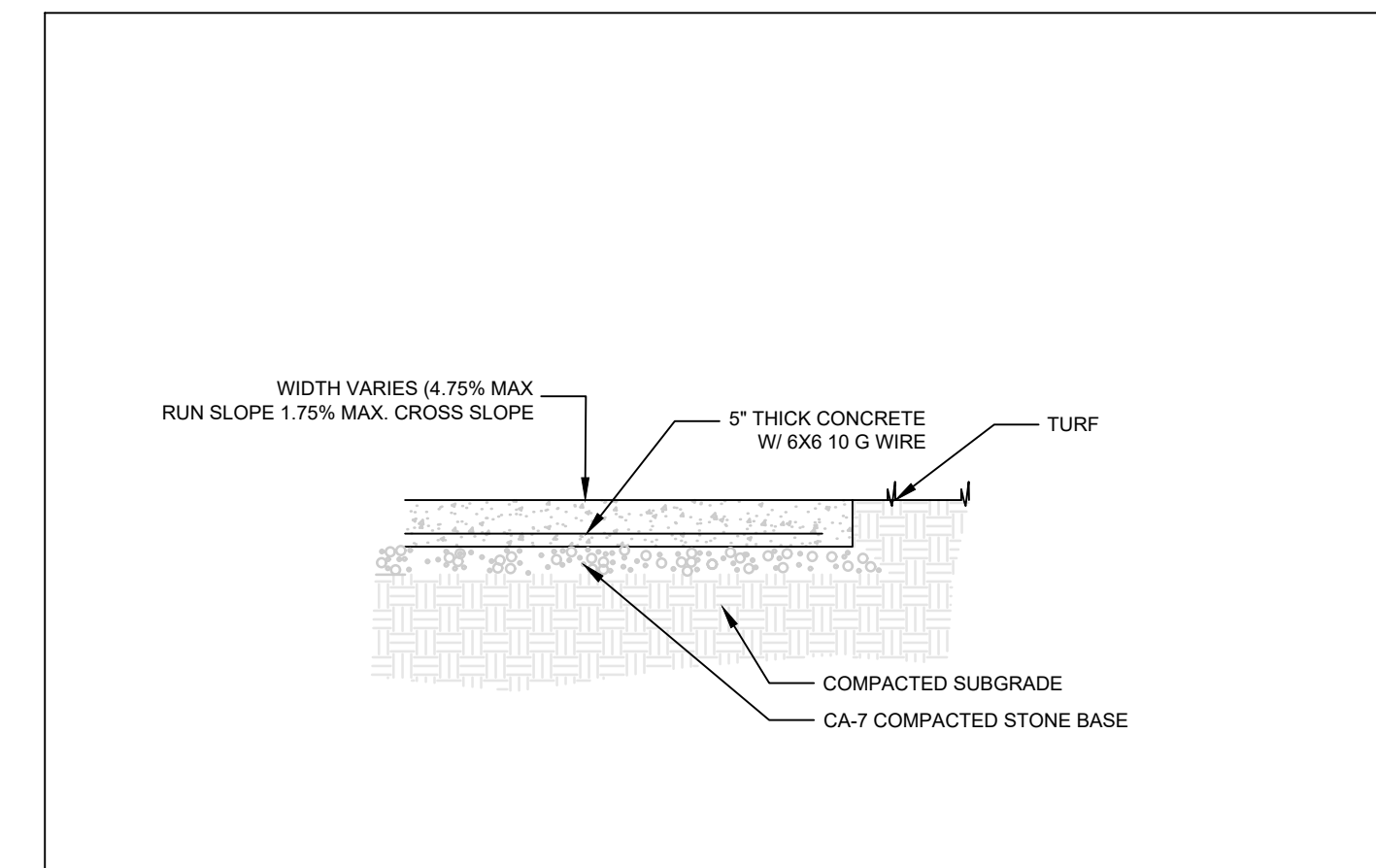
4 CONCRETE SLAB DETAIL No Scale
