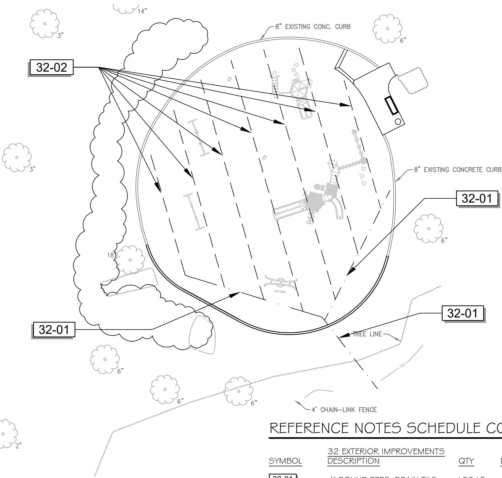
COMMUNITY PARK ENLARGED PLAYGROUND PLAN SCALE 1" = 20 FT
