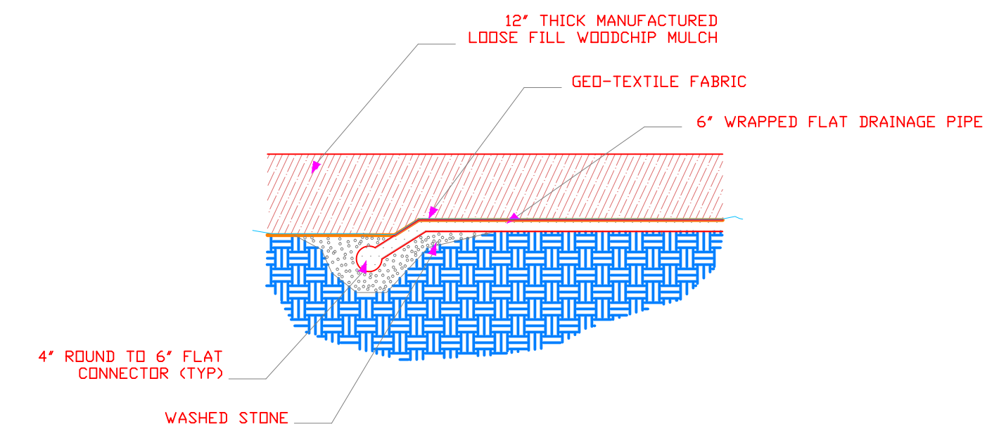
5 5 TYPICAL PLAYGROUND DRAINAGE DETAIL No Scale
