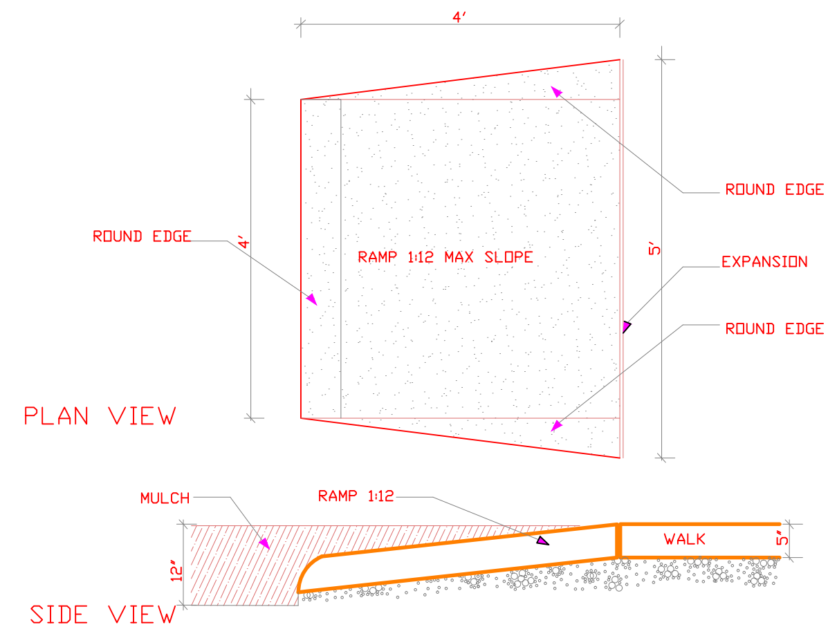
2 5 RAMP INTO PLAYGROUND DETAIL No Scale
