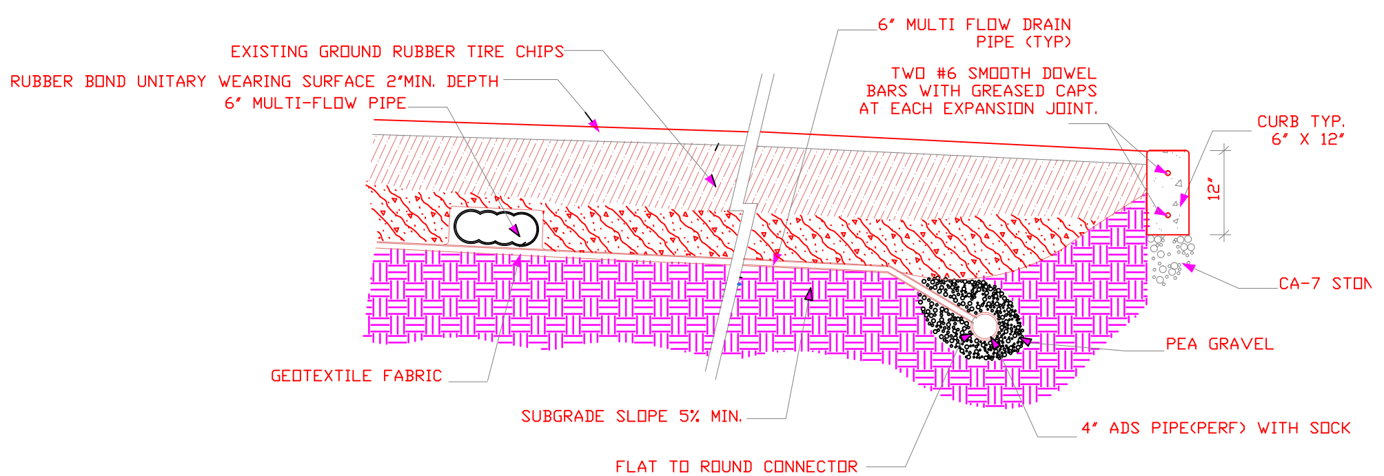
FALL SURFACE X SECTION OPTION B NO SCALE
