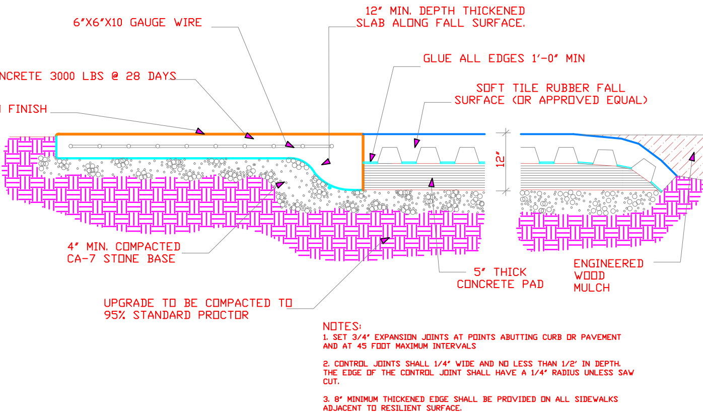
9 5 SOFTTILE FALL SURFACE DETAIL No Scale
