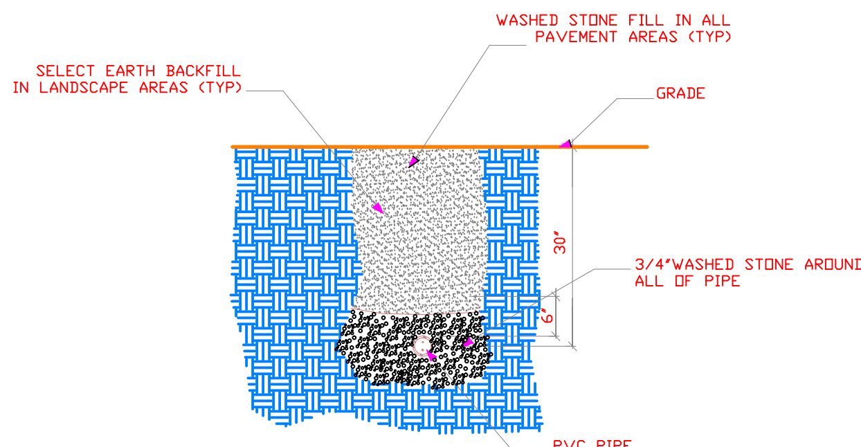
8 5 TYPICAL TRENCH DETAIL No Scale
