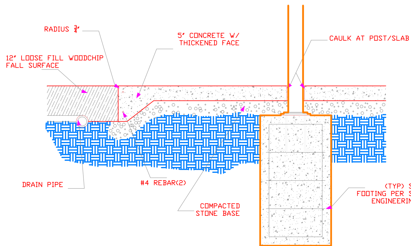
4 5 SHADE STRUCTURE COLUMN INTO SLAB DETAIL No Scale
