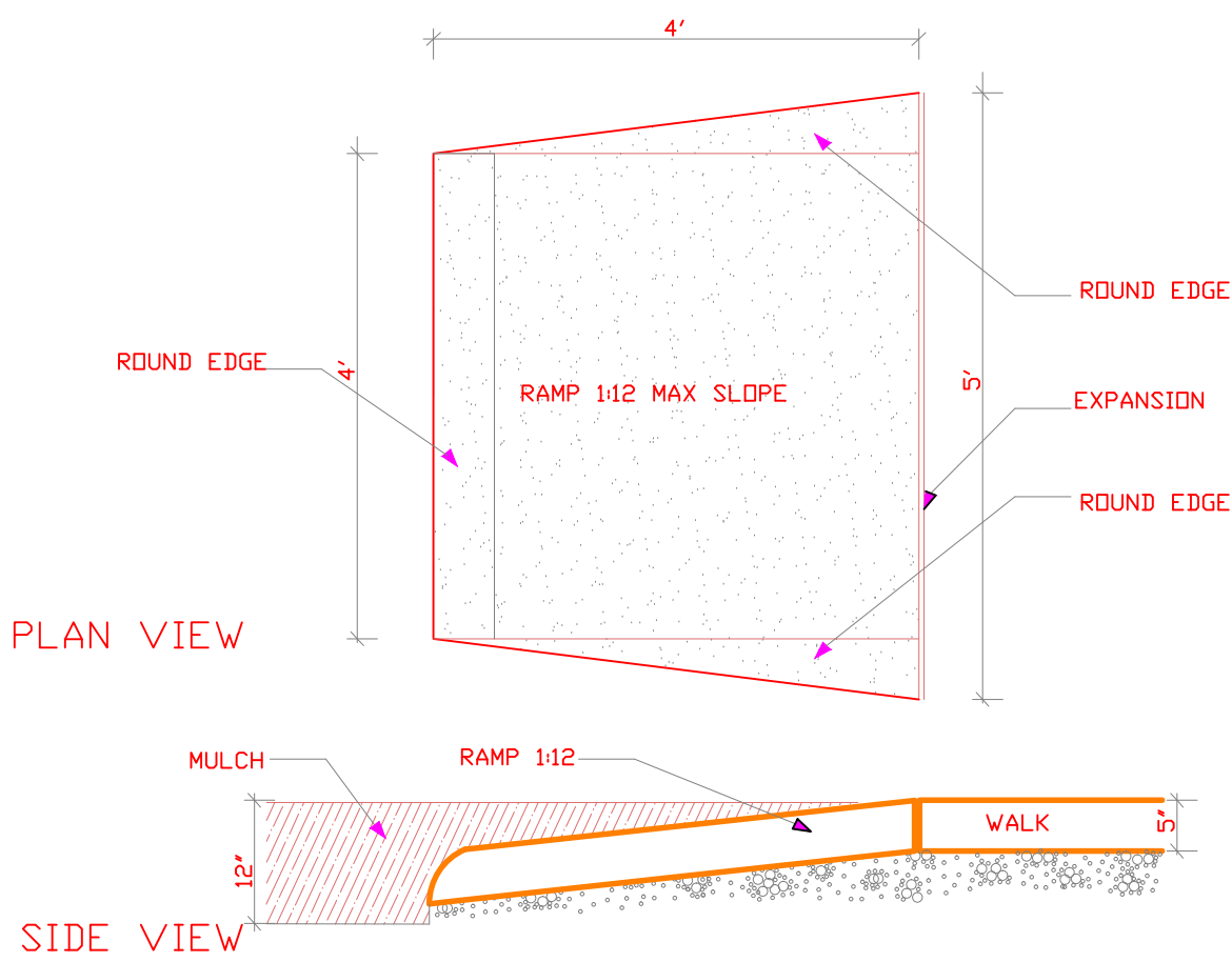
2 5 RAMP INTO PLAYGROUND DETAIL No Scale
