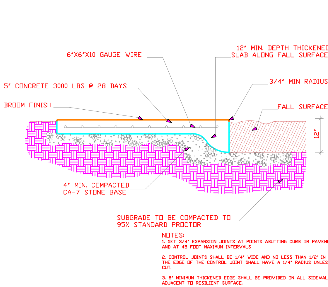
1 5 SIDEWALK DETAIL AT PLAYGROUND No Scale
