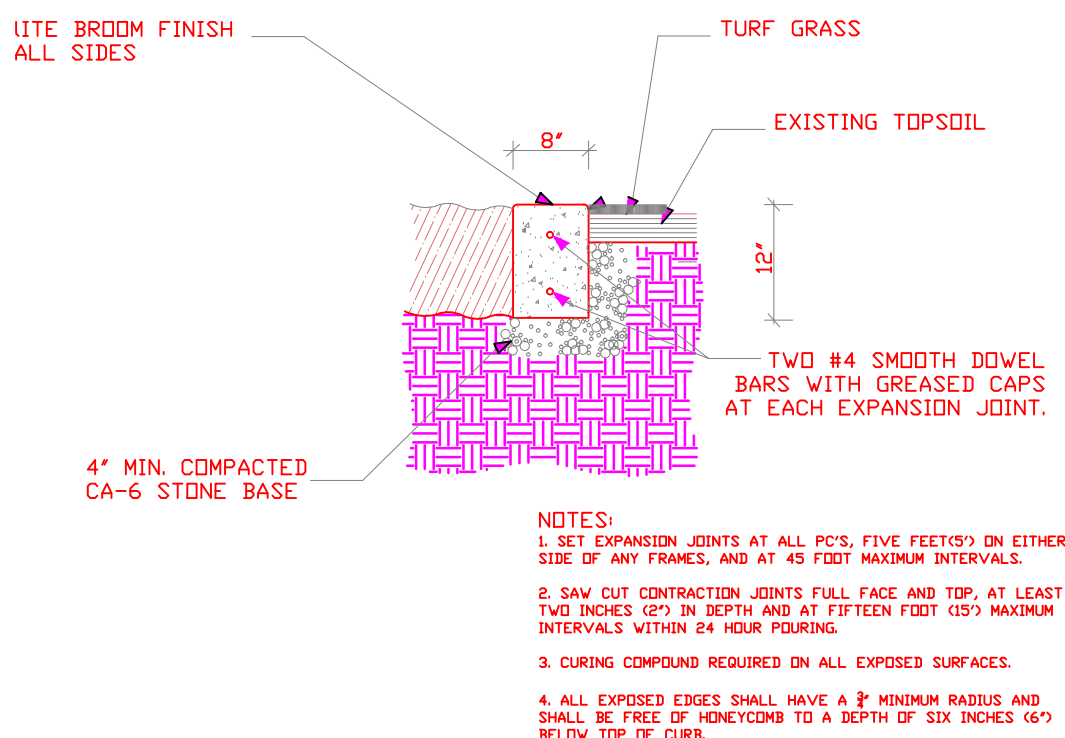
7 5 8" x 12" CONCRETE CURB DETAIL No Scale
