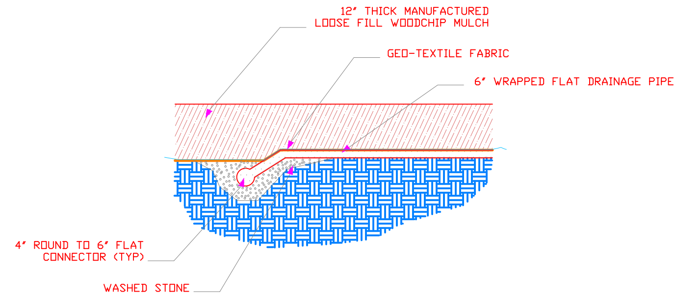
5 5 TYPICAL PLAYGROUND DRAINAGE DETAIL No Scale
