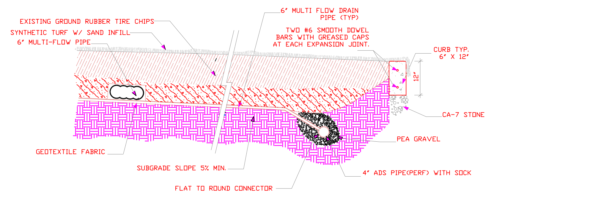
FALL SURFACE X SECTION OPTION A NO SCALE
