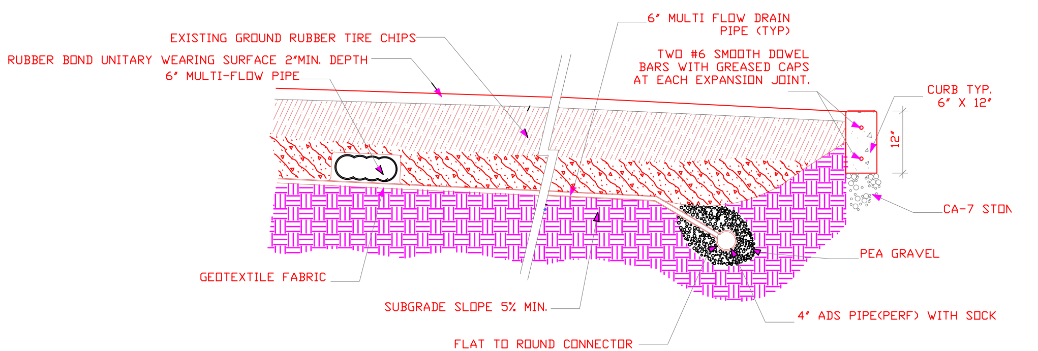
FALL SURFACE X SECTION OPTION B NO SCALE
